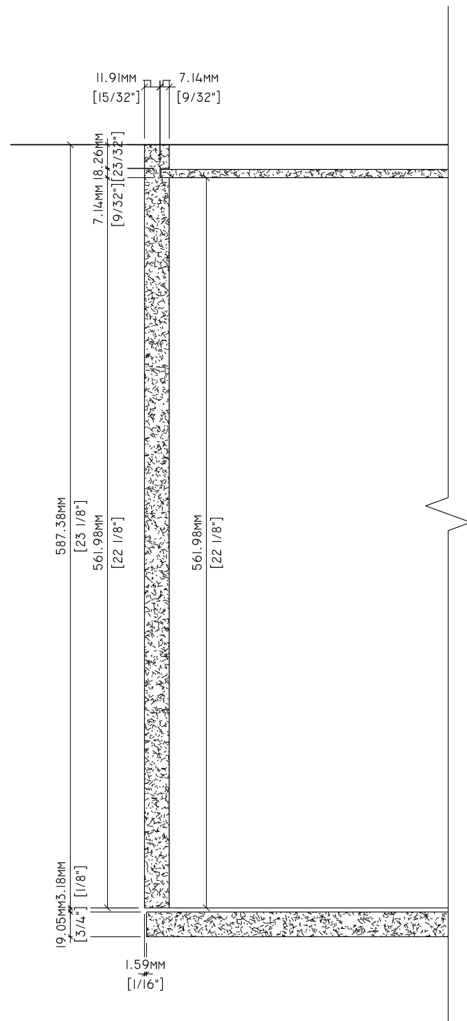
1 PLAN DETAIL T-2.4 3" = 1'-0"
