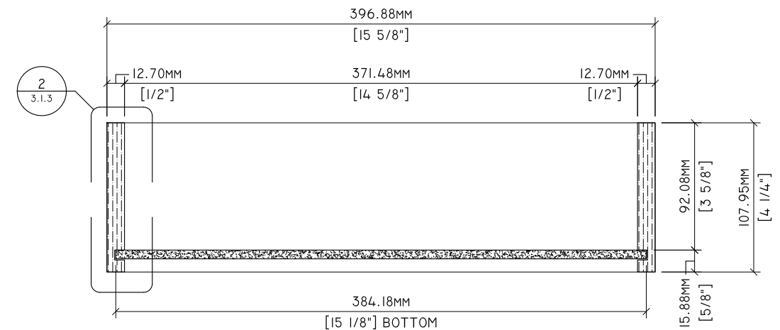
4 SECTION 5.3.2 3" = 1'-0"
