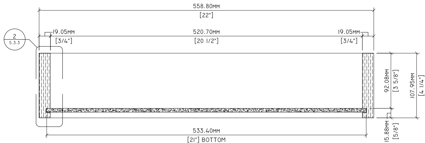
3 SECTION 5.3.2 3" = 1'-0"
