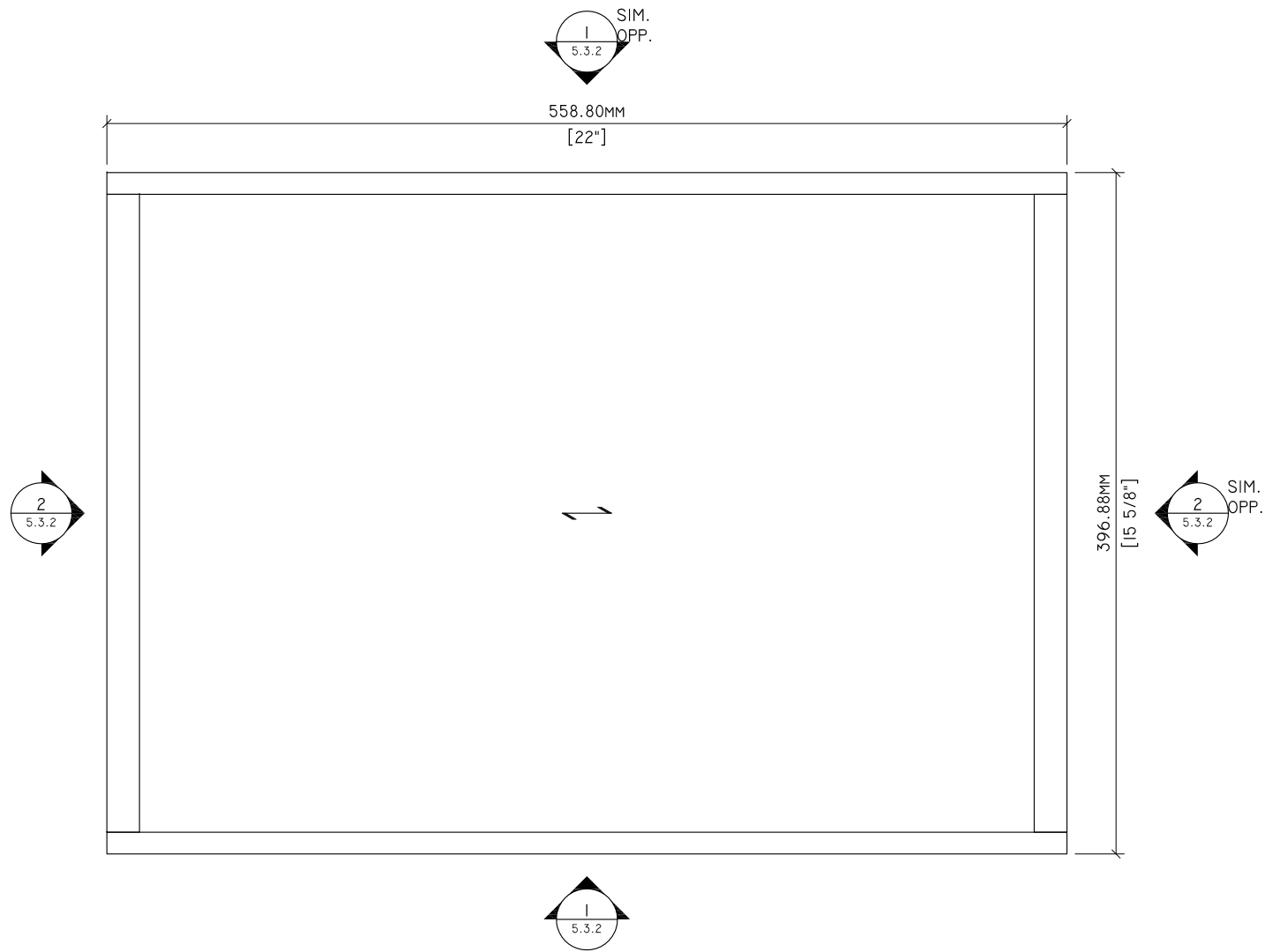
1 5.3.1 PLAN 3" = 1'-0"
