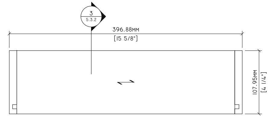
2 ELEVATION 5.3.2 3" = 1'-0"
